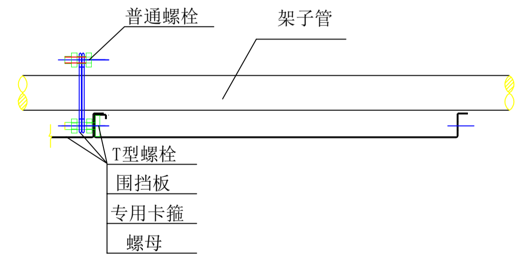
JC400组装围挡图，厚度不小于0.8mm
